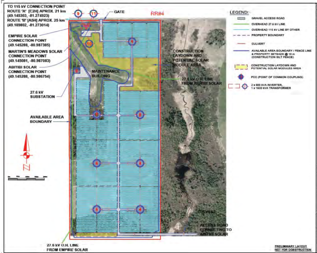
Figure 1: Site Layout
