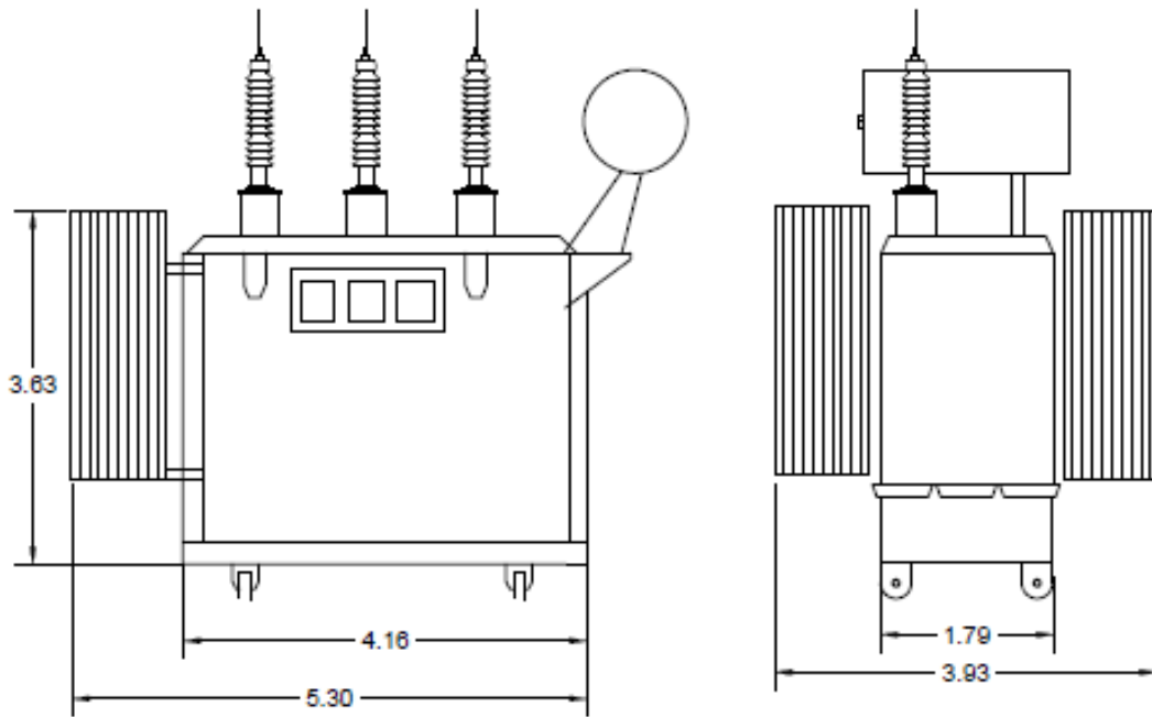
Figure B.2 27.6-kV/115-kVA/10-MVA Substation Transformer Catalogue Dimensions (metres).
